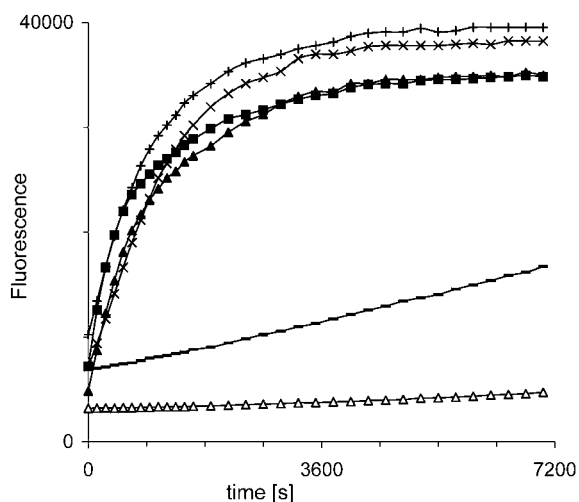
Figure 2. Esterase fluorescence assay with fluorogenic lactones 2 and 10 . ( \Delta ) 100 \mu\text{M} 2 in aqueous PBS, 10% v/v DMSO, 35 ^{\circ}\text{C} ; ( \blacktriangle ) 100 \mu\text{M} 2 with 10 \mu\text{g mL}^{-1} chirazyme E1; ( \blacksquare ) 100 \mu\text{M} 2 with 10 \mu\text{g mL}^{-1} chirazyme E2; (–) 100 \mu\text{M} 10 in aqueous PBS, 10% v/v DMSO, 35 ^{\circ}\text{C} ; (+) 100 \mu\text{M} 10 with 10 \mu\text{g mL}^{-1} chirazyme E1; (x) 100 \mu\text{M} 10 with 10 \mu\text{g mL}^{-1} chirazyme E2.
