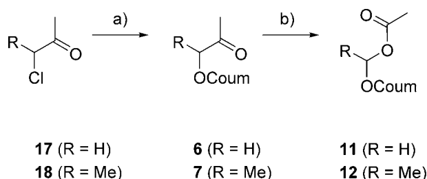
Scheme 2. Synthesis of BVMO and esterase substrates. Conditions: a) umbelliferone or p -nitrophenol, NaI, K 2 CO 3 , acetone, 25 °C, 5 h (70–97%); b) m -CPBA, NaHCO 3 , CH 2 Cl 2 , 0 °C to 25 °C, 15 h (70–87%).
