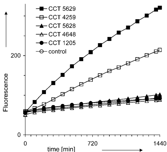
Figure 1. Whole-cell fluorescence screening of monooxygenase activity with 2-couramyloxy cyclopentanone 5 . Conditions: 100 \mu\text{M} 5 , 0.5 mg mL -1 cells, 2 mg mL -1 BSA, 20 mM aqueous borate buffer pH 8.8, 30 °C, \lambda_{\text{ex}} = 365 nm, \lambda_{\text{em}} = 460 nm. See also data in Table 1.
